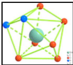
Fig. 2. The coordination environment of the Sm(III).
